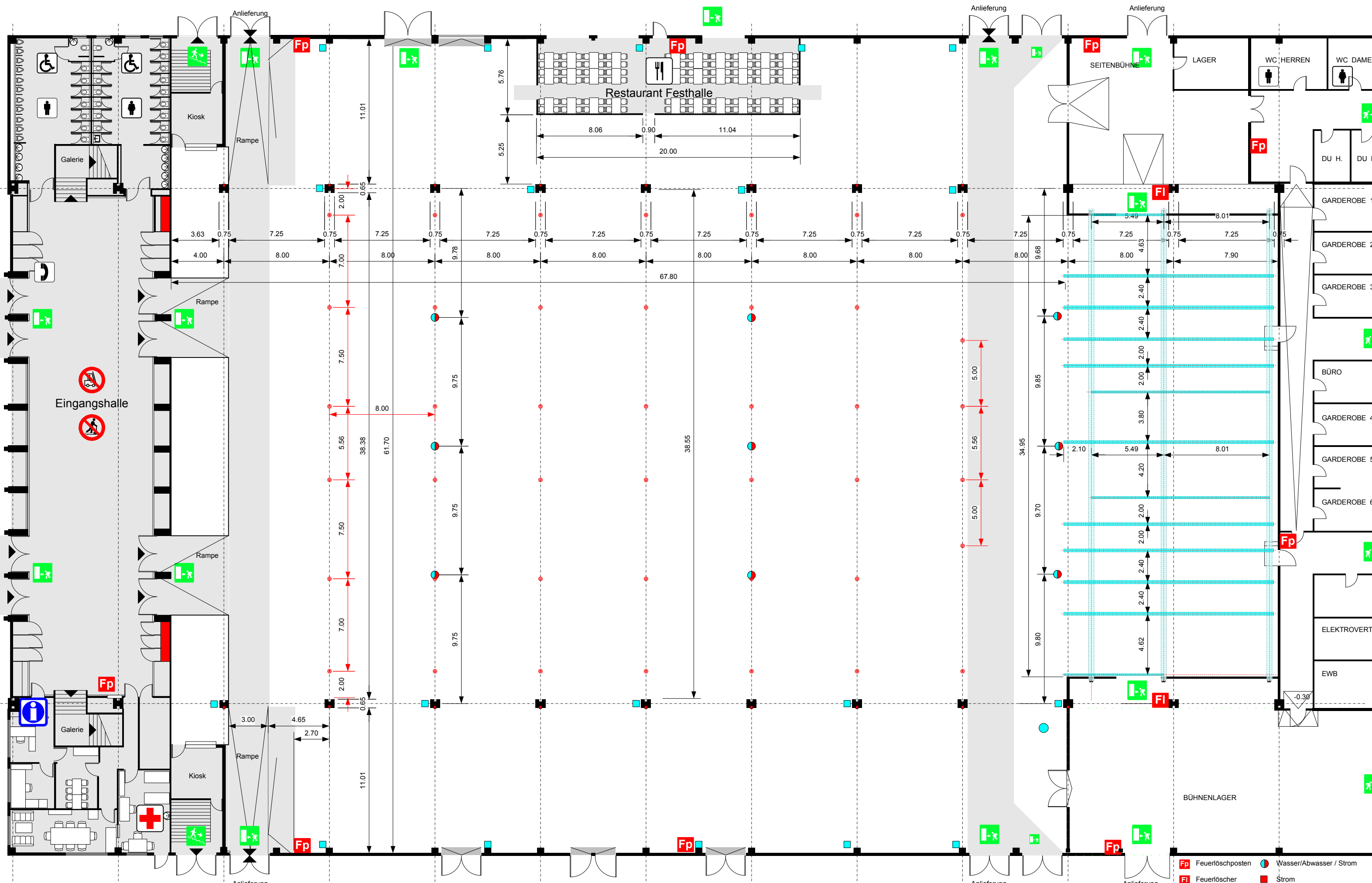
BEA bern expo Halle 310 / Festhalle Masstab 1:250 1 m 5 m 4mm = 1m
